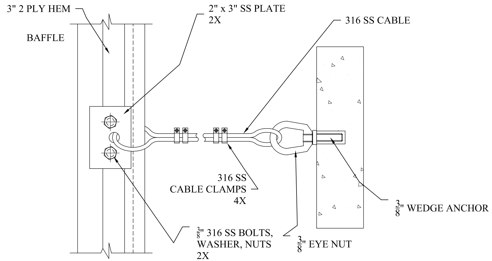
FREE END CONNECTION - CONCRETE
